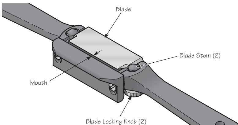
Figure 5: Adjusting the mouth.
