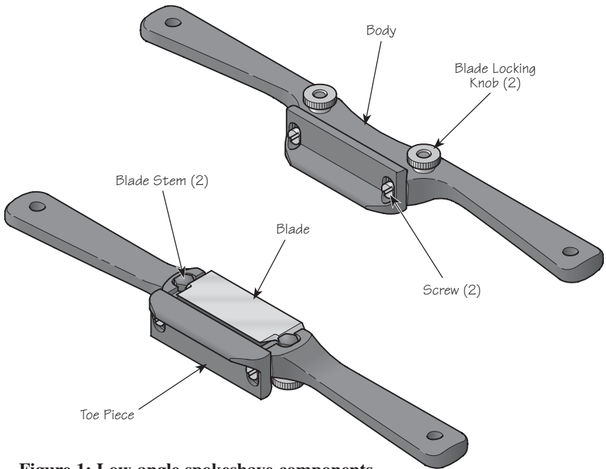
Figure 1: Low-angle spokeshave components.
