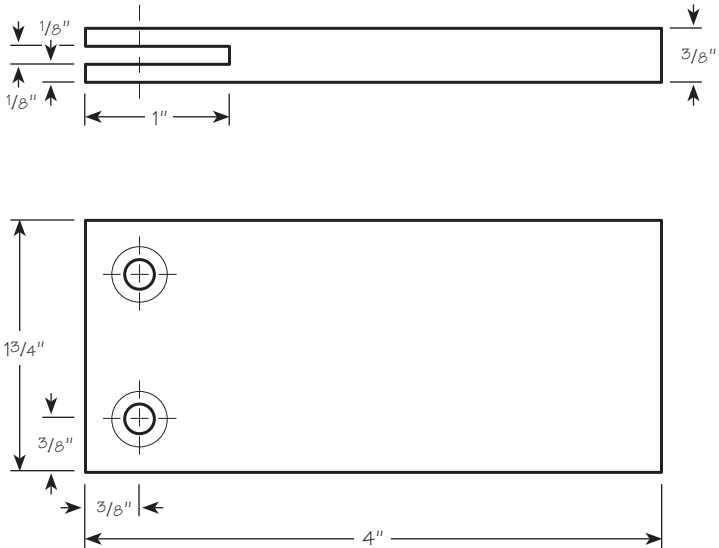
Figure 9: Blade sharpening jig plan.
