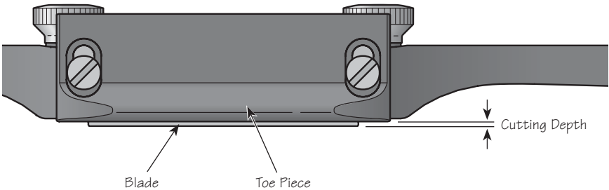
Figure 4: Adjusting the depth of cut.
