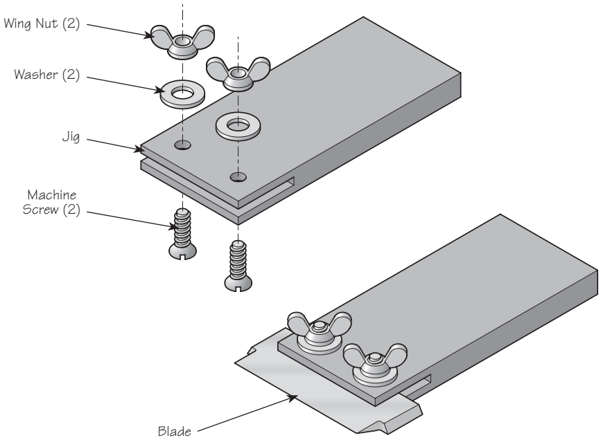
Figure 8: Blade sharpening jig.
