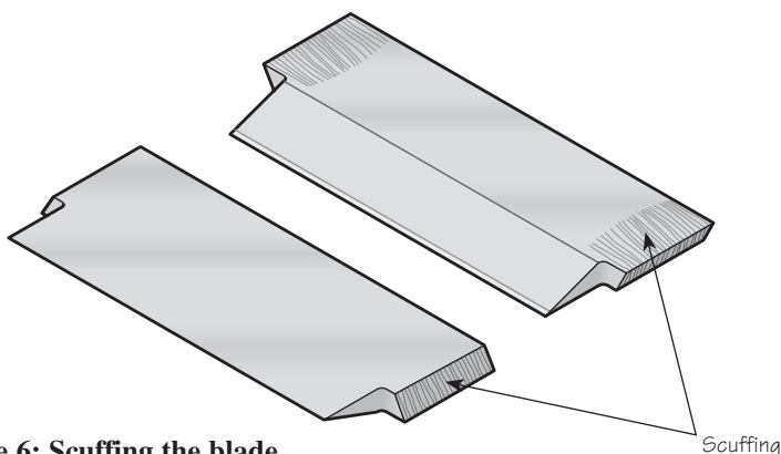
Figure 6: Scuffing the blade.
